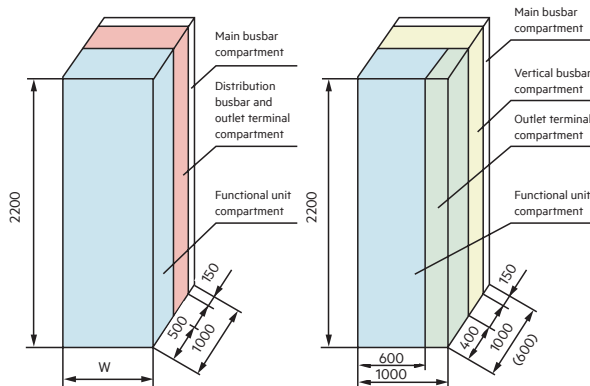
a.PC Cabinet
