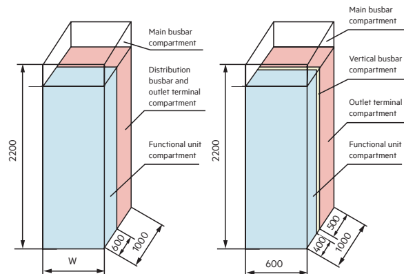
c.PC Cabinet
