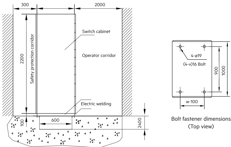
Installation diagram
