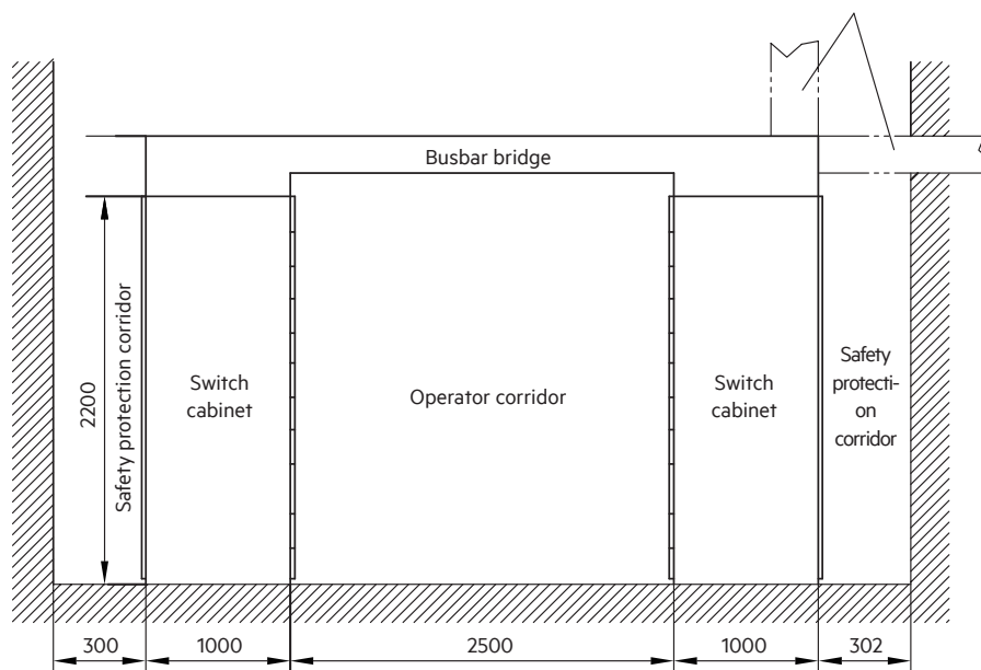
Installation diagram
