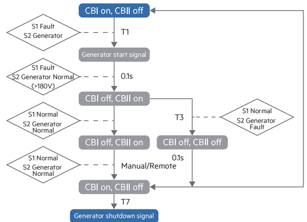
Mains - generator, self casting non self restoring mode 2:
