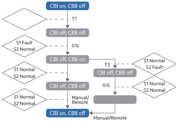
mains - mains, self-feed no self-recovery mode 1:
