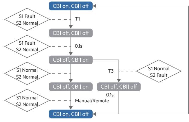
Mains - Mains, self-feed no self-recovery mode 2:
