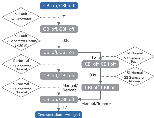
mains - generator, self-feed no self-recovery mode 1:
