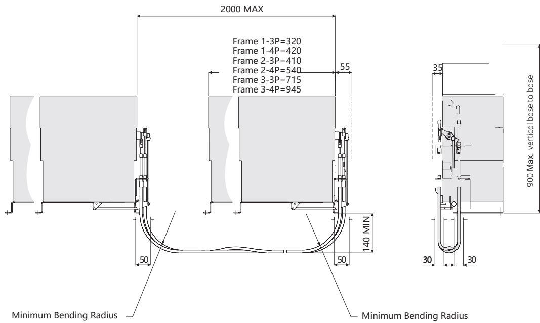
2-way mechanical interlocking mechanism / Fixed pattern - Front connection / Rear connection
