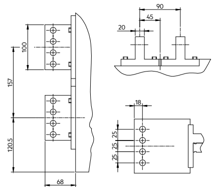
Standard rear vertical connection busbar up to 6400A
