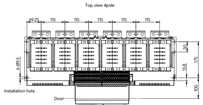
Standard rear vertical connection busbar up to 6400A
