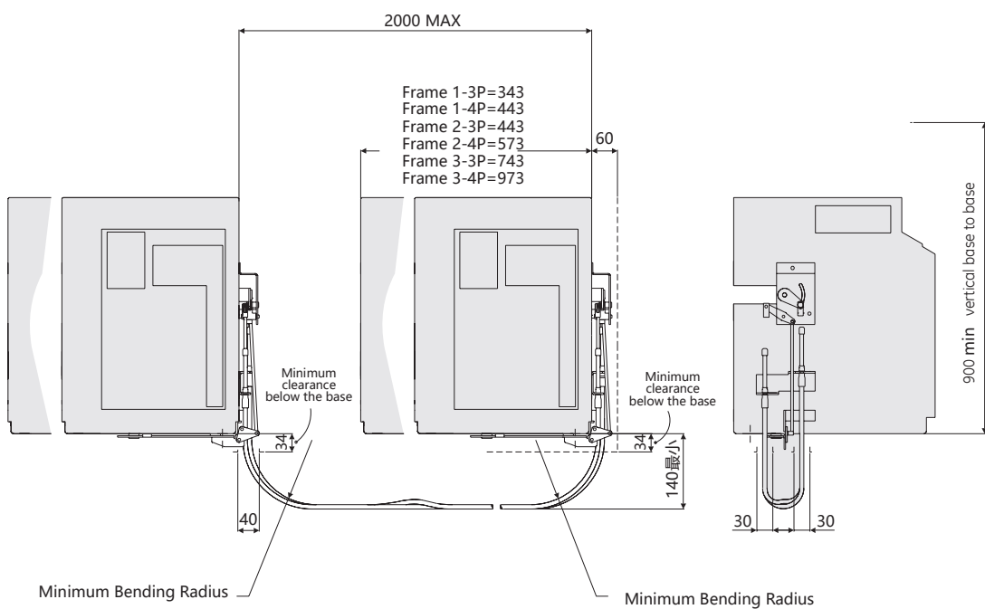
2-way mechanical interlocking mechanism / Draw-out pattern - Front connection / Rear connection
