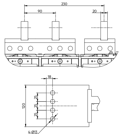
Standard rear vertical connection busbar up to 6400A
