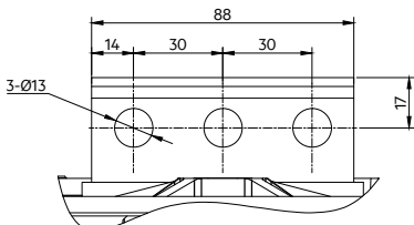
Standard rear vertical connection busbar up to 5000A
