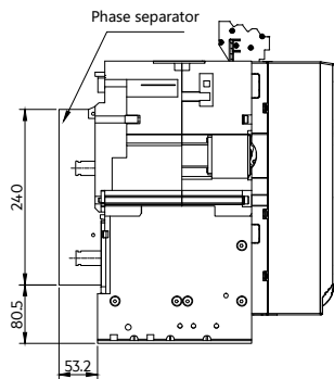
MEX 1&2 standard isolation phase separator dimension for fixed pattern
