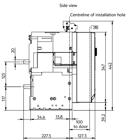
Standard rear vertical connection busbar up to 5000A
