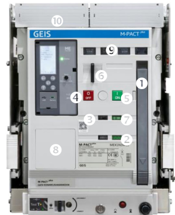
Front panel of circuit breaker
