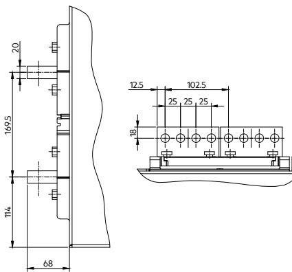
Standard rear horizontal connection busbar up to 5000A
