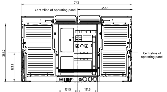
Front view 3pole
