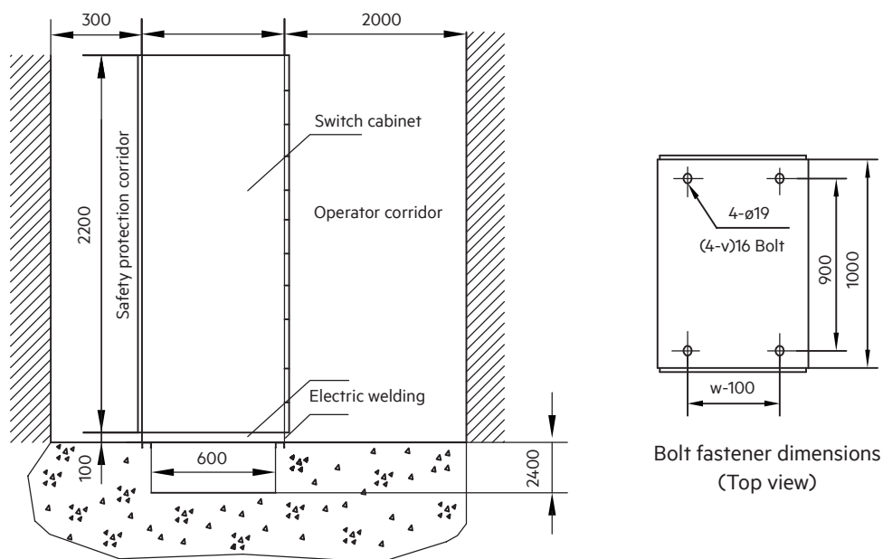
Installation diagram
