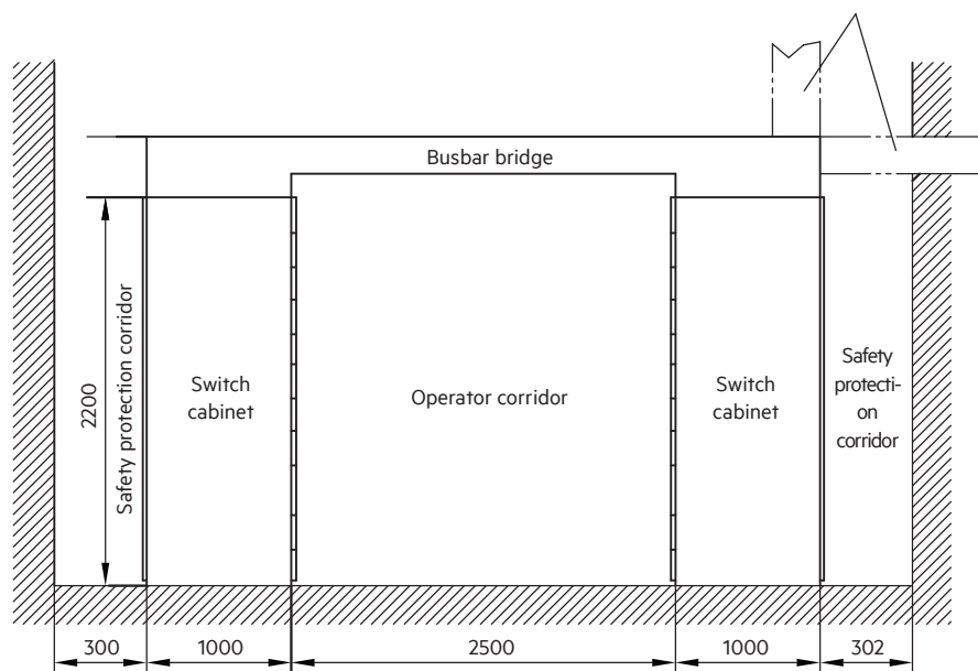
Installation diagram
