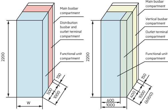
a.PC Cabinet
