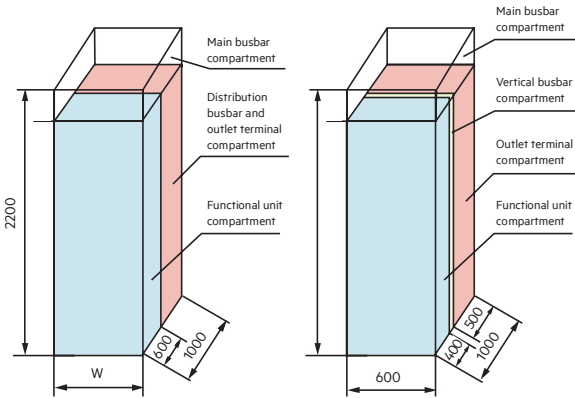
c.PC Cabinet
