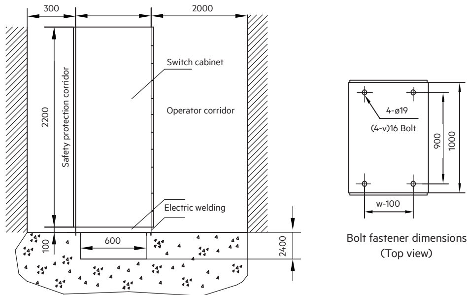
Installation diagram
