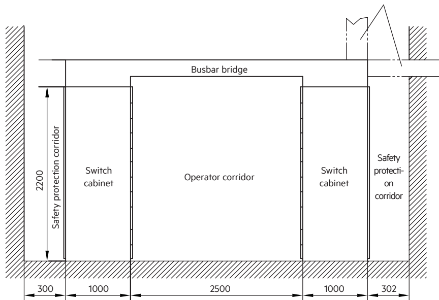
Installation diagram
