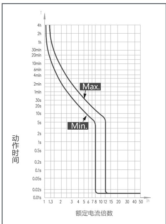
GB/GE400 Time-Current Curves, TM
