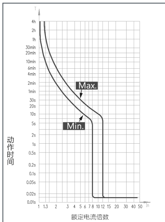
GB/GE250 Time-Current Curves, TM
