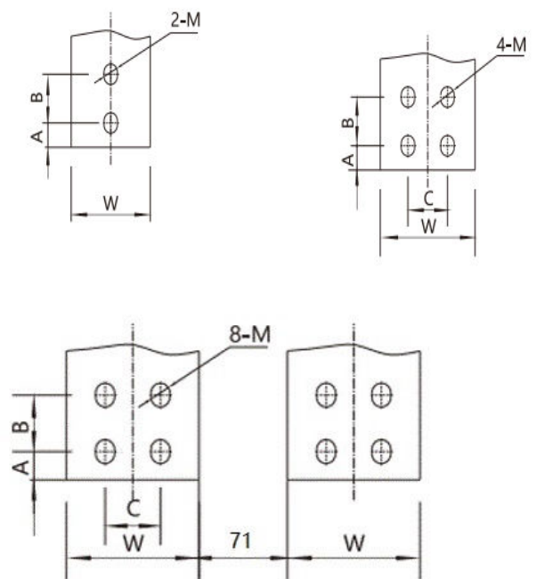
double-layer busway
